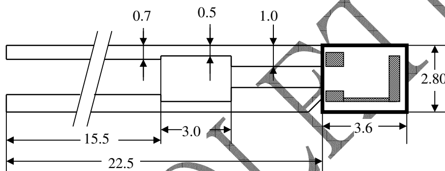
Humidity Sensor type SMTHS10
