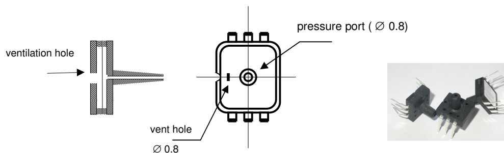
Fig. 2, principle of a gauge type pressure sensor
