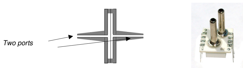
Fig 4, Principle of differential pressure sensor.
